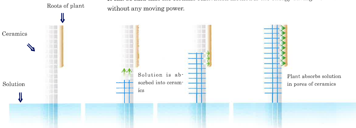
Figure of supplying solution of cultivation by ceramics
